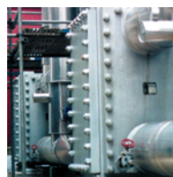
Vertical Compabloc for liquid/liquid heat recovery
