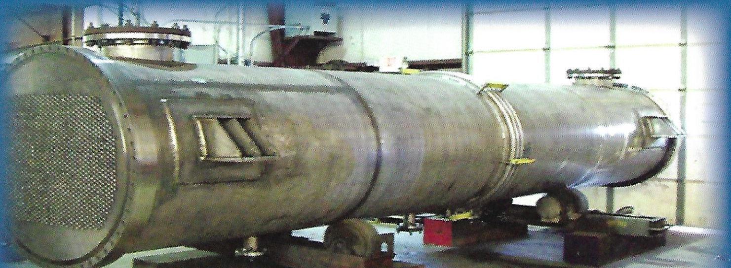
Alloy 625-Alloy 800 Gas Expander Heater
